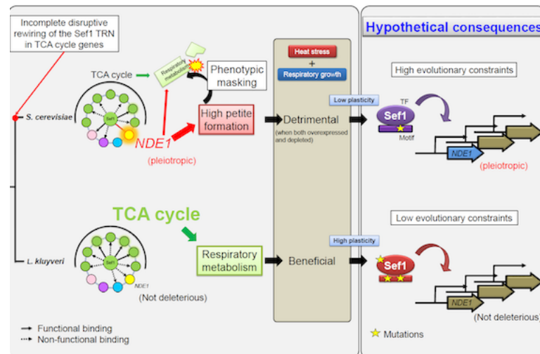
A New Evolutionary Trajectory of Transcriptional Rewiring: Incomplete Rewiring Can Still Dramatically Overturn the Phenotypic Trait
